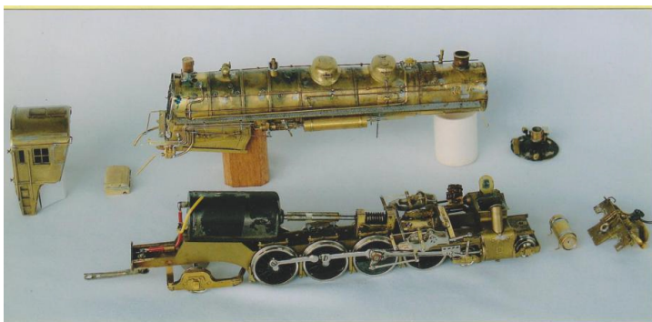
LEFT: Photos of Kyle's brass model prior to painting. Note the working Baker valve gear in the middle photo by Kyle Gardiner, 2004
